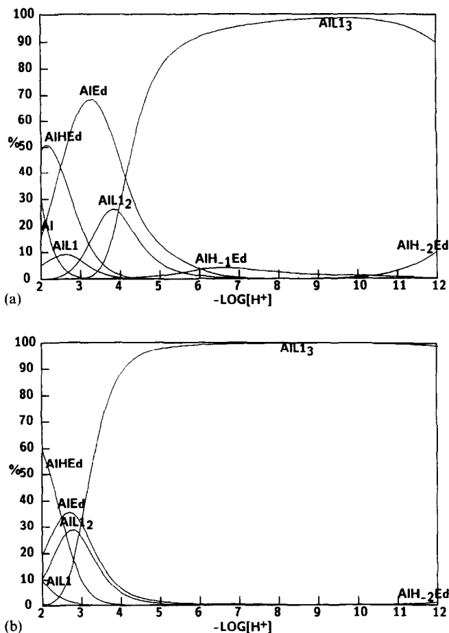
Fig. 6. (a) Relative molar concentrations of complex species formed from 1.0 \times 10^{-3} M Al(III), 3.0 \times 10^{-3} M 1,2-dimethyl-3-hydroxy-4-pyridinone (L1), and 1.0 \times 10^{-3} M EDTA. L1=HL; EDTA= H_4L =Ed; T=25.0^\circ\text{C} ; \mu=0.10 (KCl). (b) As (a), except at 100 times the concentration.
