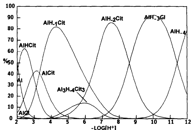
Fig. 5. Relative molar concentrations of complex species formed from 1.0 \times 10^{-3} M Al(III) (=100%), 1.0 \times 10^{-2} M citric acid, and 1.0 \times 10^{-2} M gluconic acid. Citric acid = \text{H}_3\text{L} = \text{Cit} ; gluconic acid = \text{HL} = \text{Gl} ; T = 25.0^\circ\text{C} ; \mu = 0.10 (KCl).
