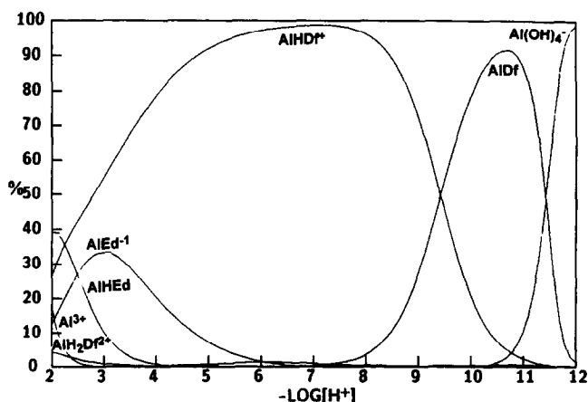
Fig. 8. DFO more effective than EDTA for binding Al(III). EDTA = H_4E ; DFO = H_3L or H_4L^+ ; Al^{3+} = M^{3+} . Total concentrations of components, T_{\text{EDTA}} = T_{\text{DFO}} = T_{\text{Al(III)}} = 0.0010 M; T = 25.0^\circ\text{C} ; \mu = 0.100 M (KCl).
